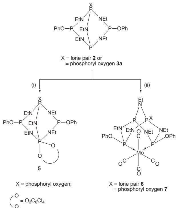
Scheme 2 (i) Tetrachloro-1,2-benzoquinone, benzene, 0 °C; (ii) [Mo(CO) 4 (nbd)], light petroleum, 50–60 °C
