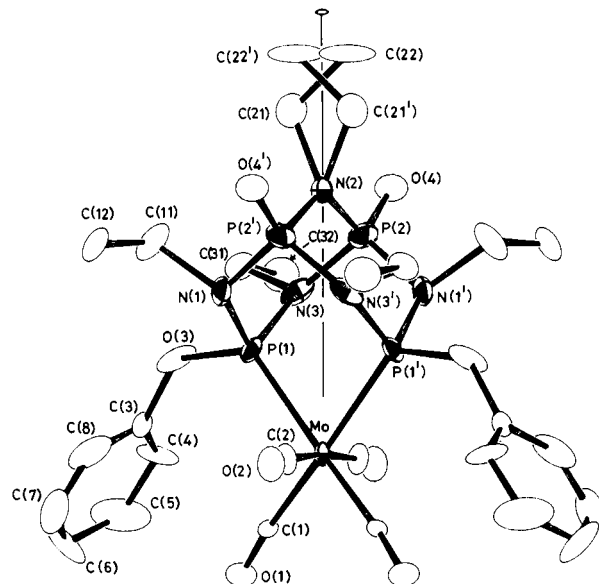
Fig. 4 Molecular structure of 7 . 'Rotational disorder' of ethyl group at N(2) and 'statistical disorder' of oxygen at P(2) and P(2') are shown
