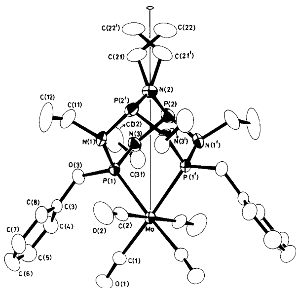
Fig. 3 A perspective view of molecule 1 in the unit cell of complex 6 . 'Rotational disorder' of ethyl group at N(2) is shown
